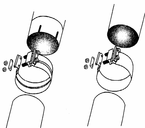
EXHAUST CLAMPS HARDWARE SETS
