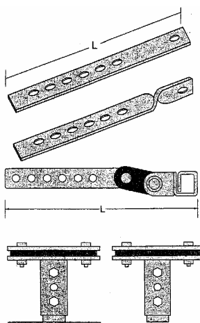
MULLER BRACKETS & HANGERS
