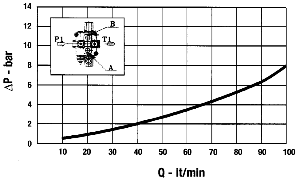
Pressure Drop with Spool In Working Position
